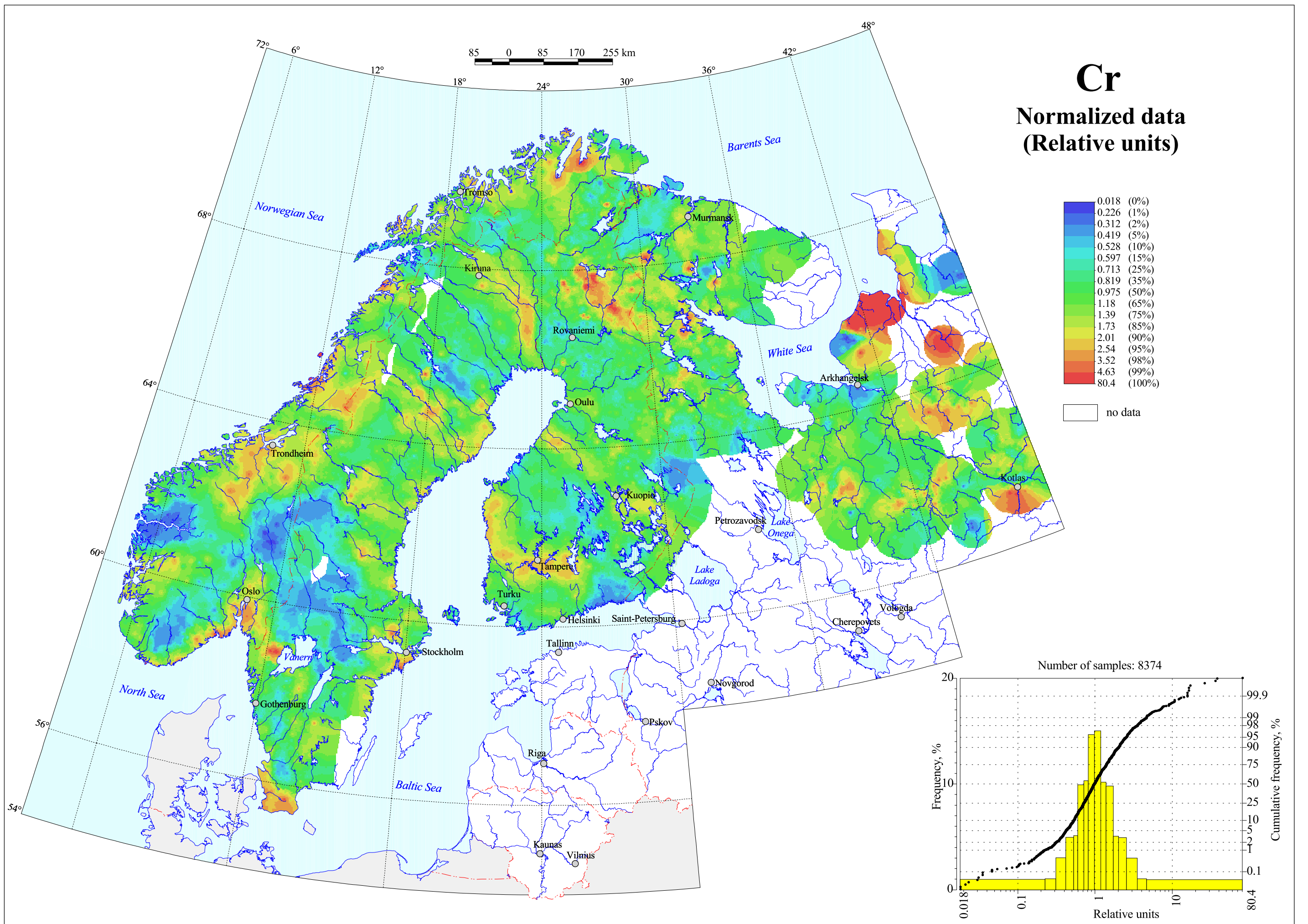
Chromium in Till, Grain Size <0.06 mm
